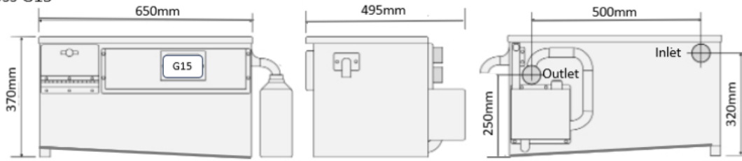
Grease Boss G15
