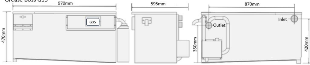
Grease Boss G35
